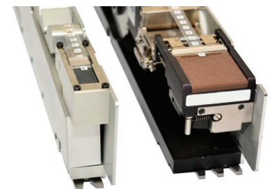
ILP-30 Label Feeder 30mm wide
