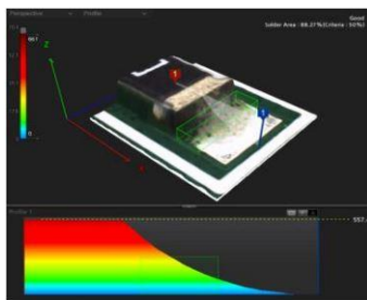
3D Solder Fillet Inspection
