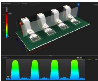
3D Gull-Wing Co-Planarity Inspection
